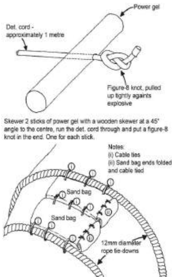
Fig. 3. Configuration of Powergel and detonation chord.
